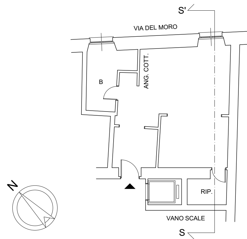
PLANIMETRIA POST OPERAM rapp. 1:100
